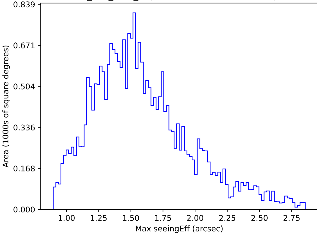
smc_lmc_v3.3_10yrs Yr 1 r band: Max seeingEff
