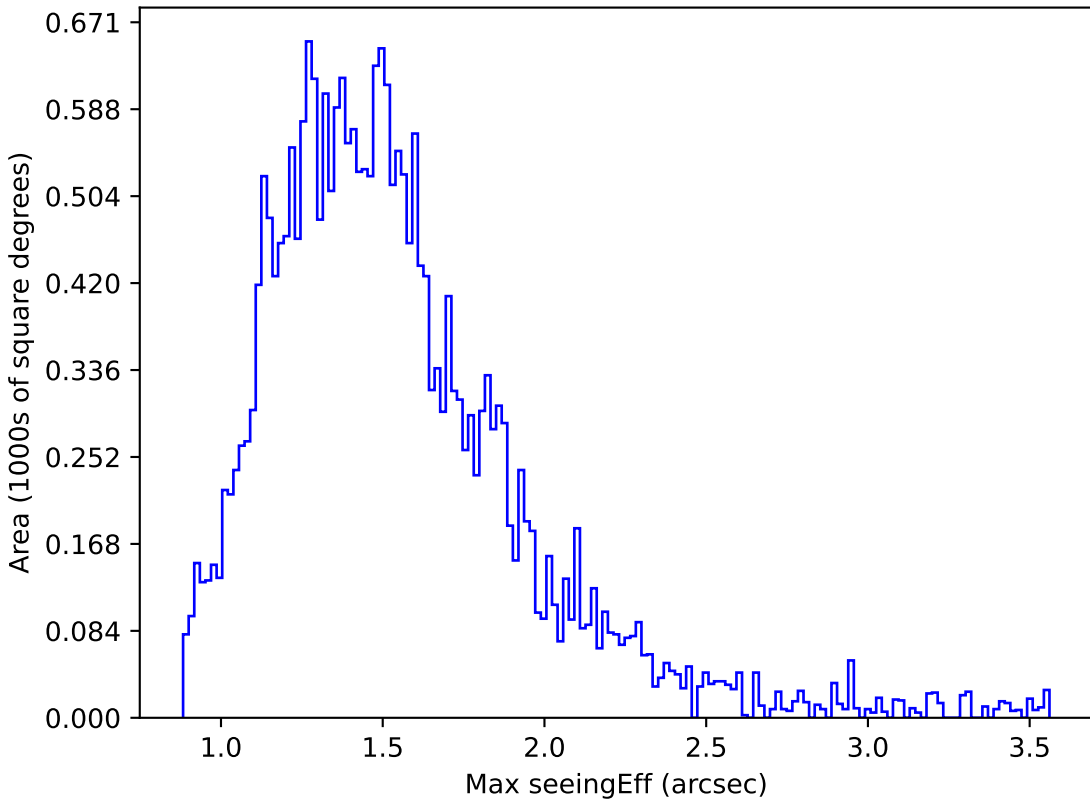
smc_lmc_v3.3_10yrs Yr 1 g band: Max seeingEff
