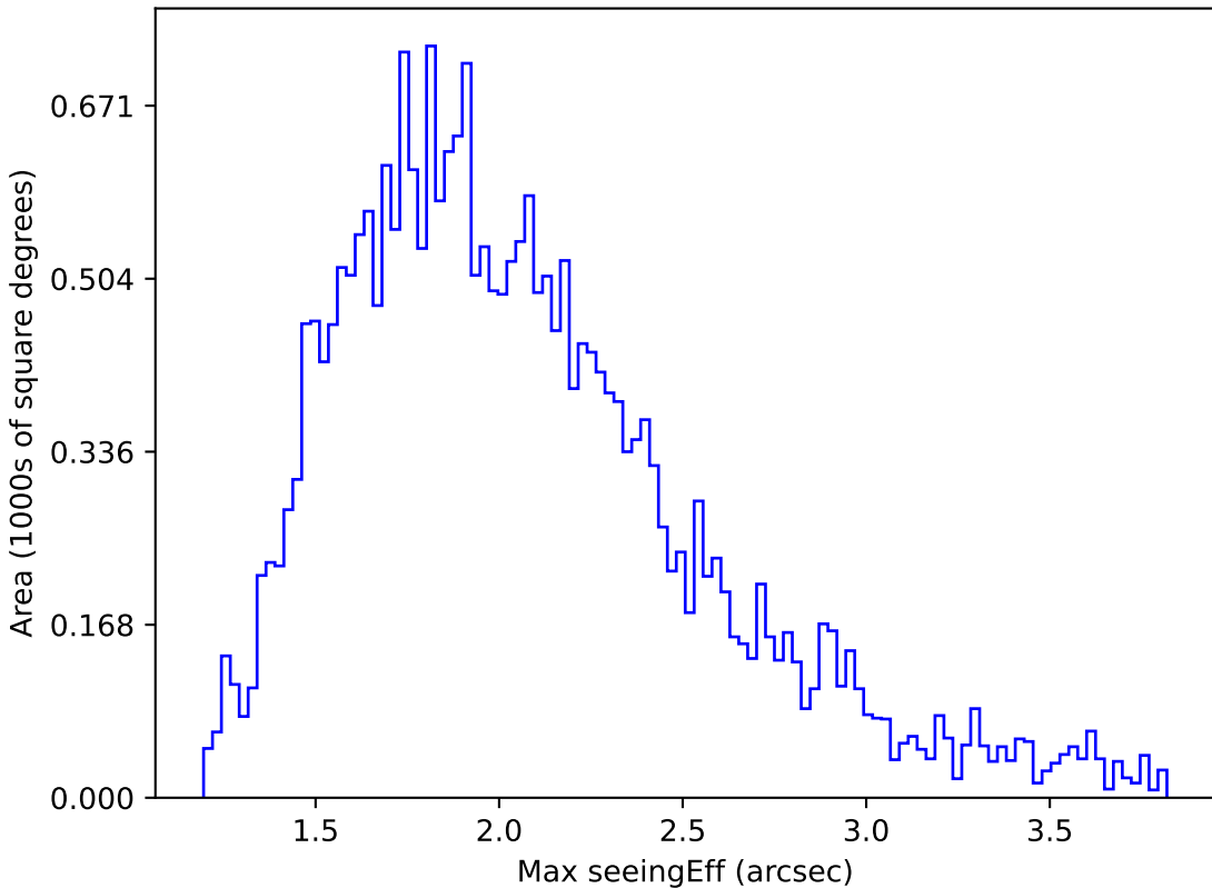
smc_lmc_v3.3_10yrs Yr 1 all bands: Max seeingEff
