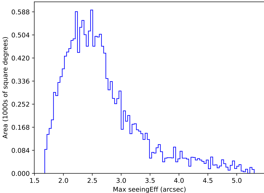
smc_lmc_v3.3_10yrs WFD z band: Max seeingEff
