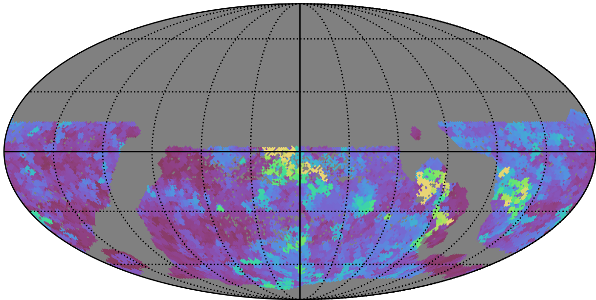
smc_lmc_v3.3_10yrs WFD y band: Max seeingEff
