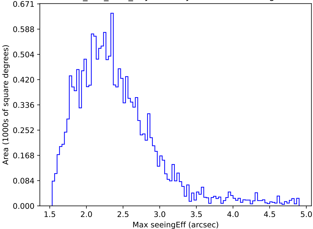
smc_lmc_v3.3_10yrs WFD y band: Max seeingEff
