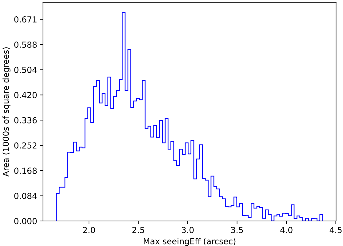
smc_lmc_v3.3_10yrs WFD u band: Max seeingEff
