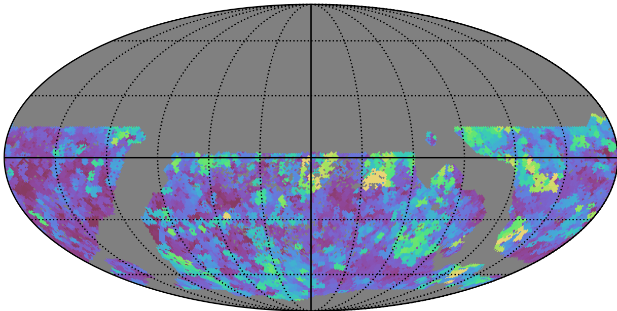
smc_lmc_v3.3_10yrs WFD r band: Max seeingEff
