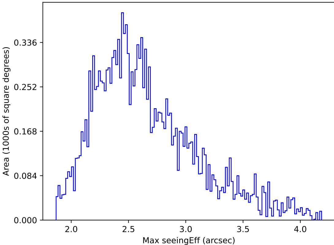
smc_lmc_v3.3_10yrs WFD r band: Max seeingEff
