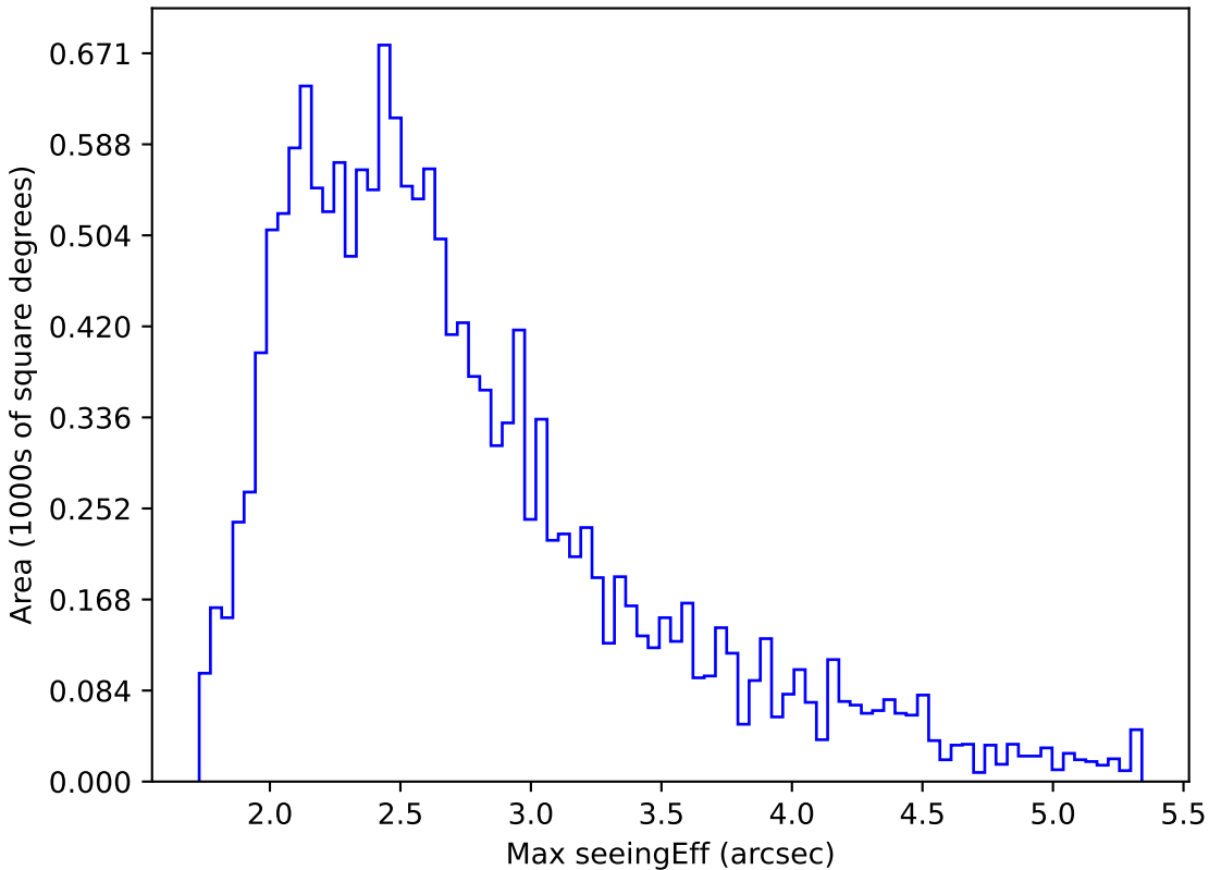
smc_lmc_v3.3_10yrs WFD i band: Max seeingEff
