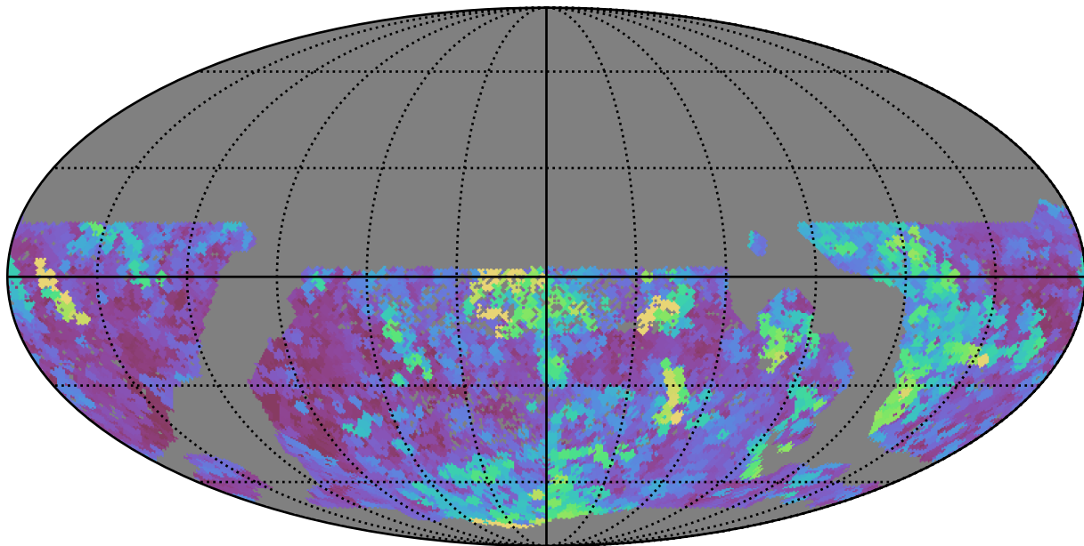
smc_lmc_v3.3_10yrs WFD all bands: Max seeingEff
