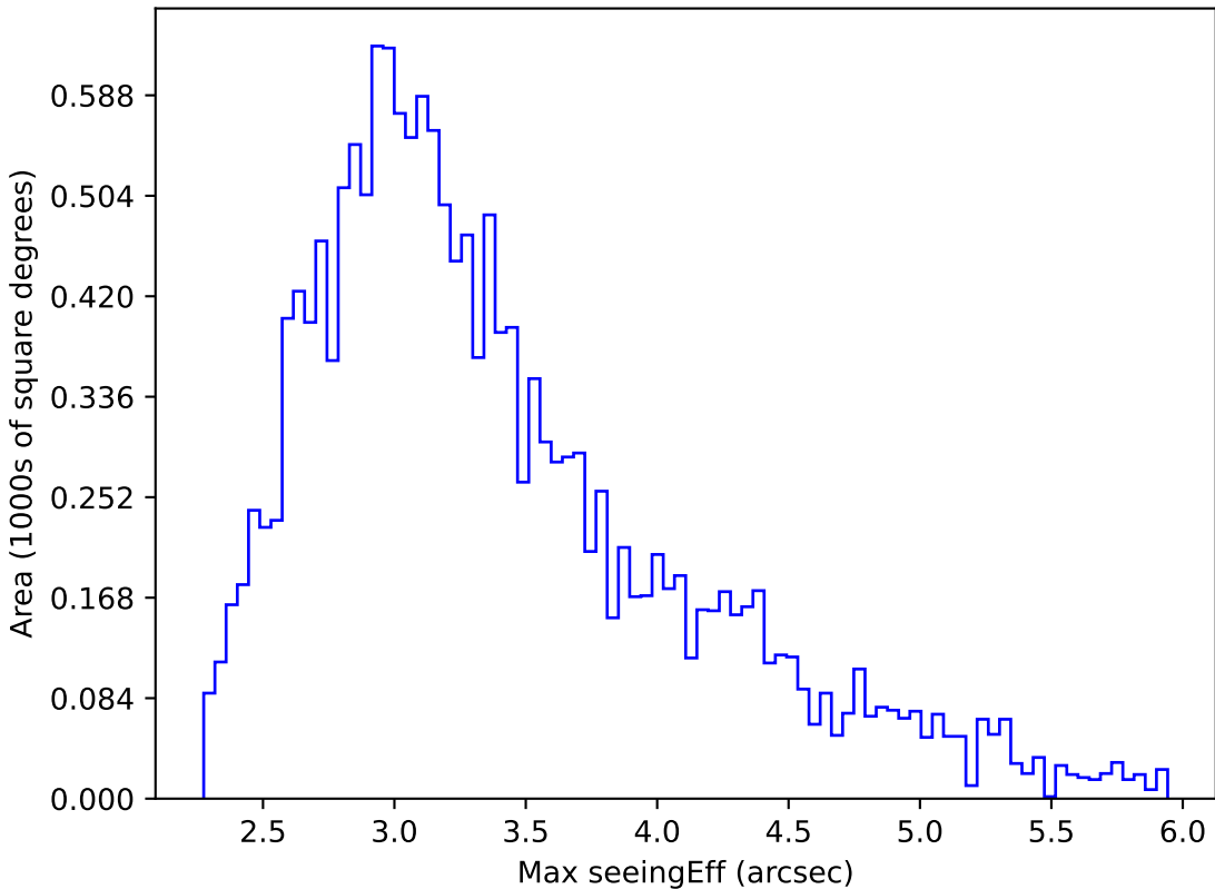
smc_lmc_v3.3_10yrs WFD all bands: Max seeingEff
