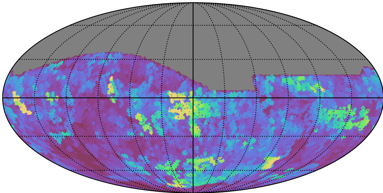
smc_lmc_v3.3_10yrs All sky z band: Max seeingEff
