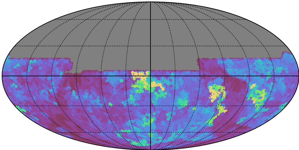
smc_lmc_v3.3_10yrs All sky y band: Max seeingEff
