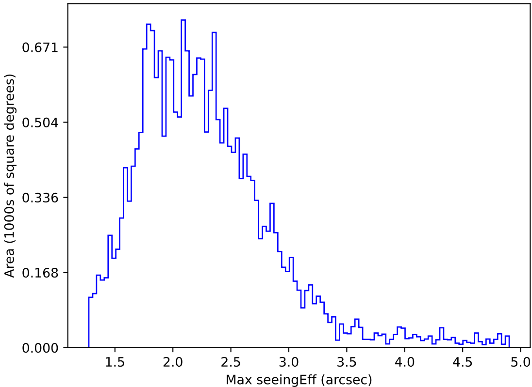
smc_lmc_v3.3_10yrs All sky y band: Max seeingEff
