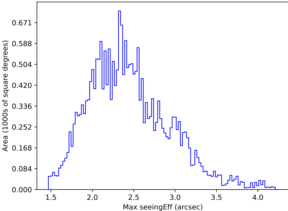
smc_lmc_v3.3_10yrs All sky u band: Max seeingEff
