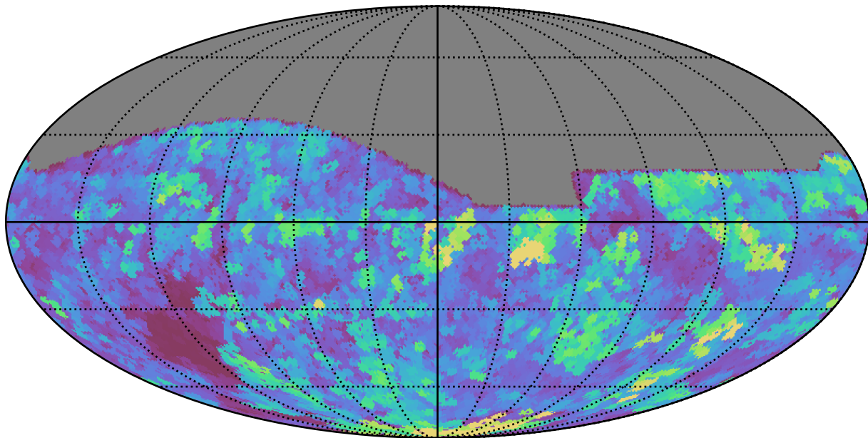
smc_lmc_v3.3_10yrs All sky r band: Max seeingEff
