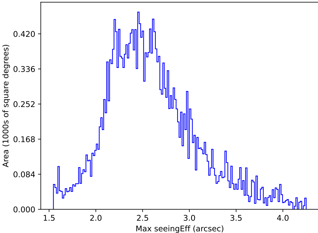
smc_lmc_v3.3_10yrs All sky r band: Max seeingEff
