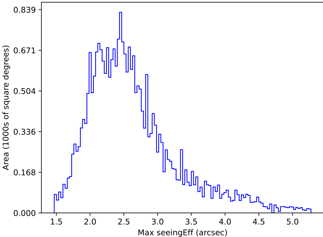
smc_lmc_v3.3_10yrs All sky i band: Max seeingEff
