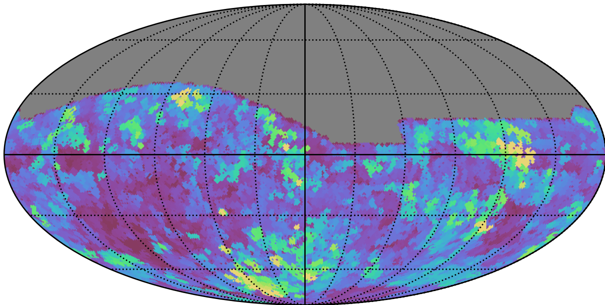
smc_lmc_v3.3_10yrs All sky g band: Max seeingEff
