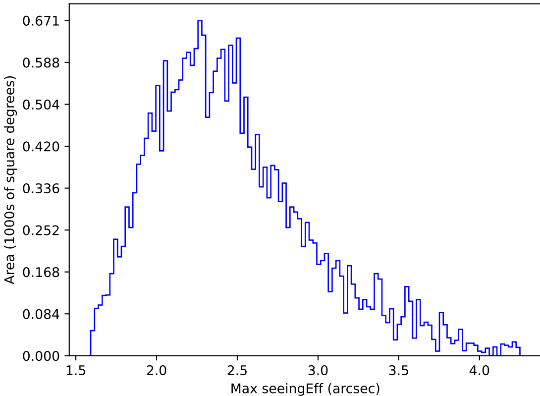
smc_lmc_v3.3_10yrs All sky g band: Max seeingEff
