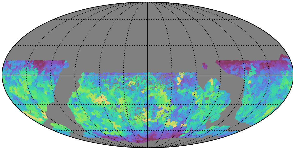
smc_lmc_v3.3_10yrs WFD z band: Max saturation_mag
