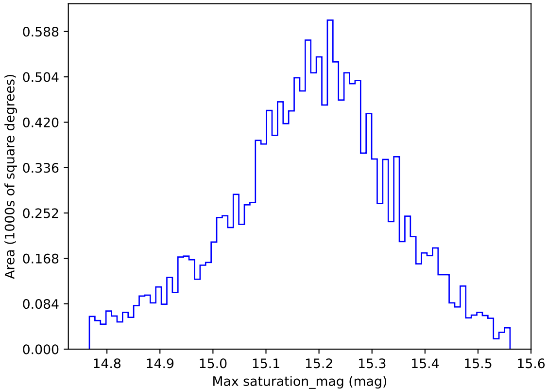
smc_lmc_v3.3_10yrs WFD z band: Max saturation_mag
