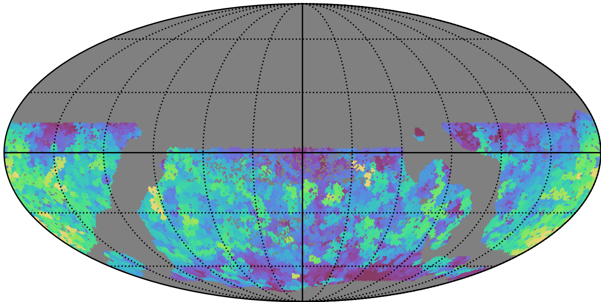
smc_lmc_v3.3_10yrs WFD u band: Max saturation_mag
