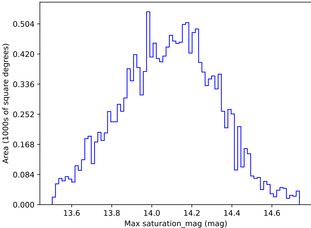
smc_lmc_v3.3_10yrs WFD u band: Max saturation_mag
