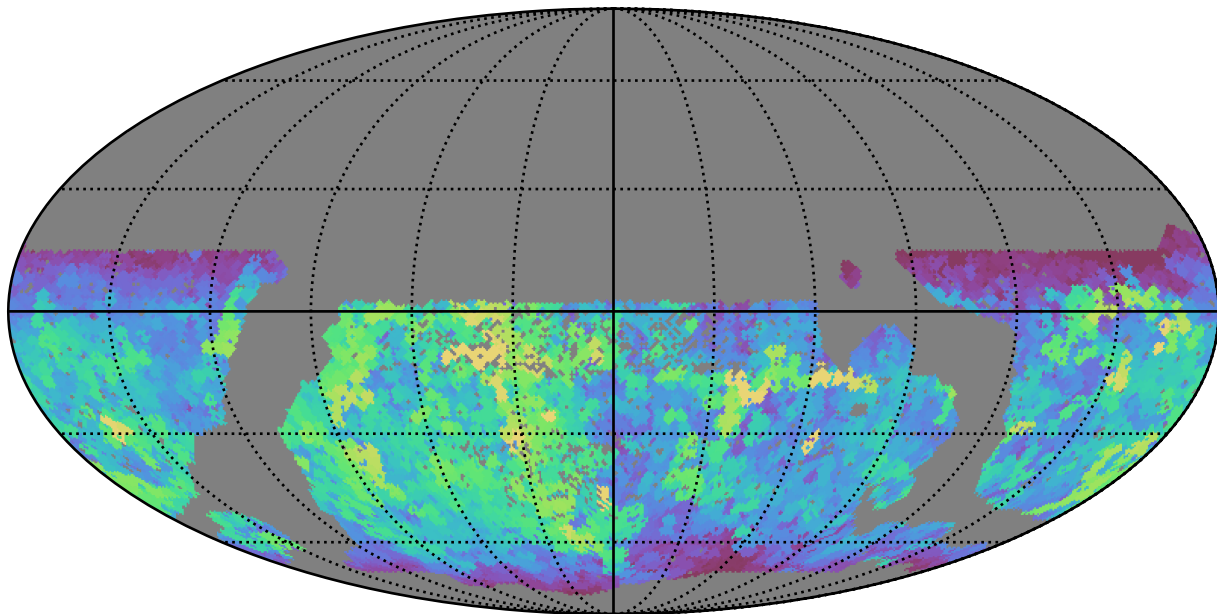
smc_lmc_v3.3_10yrs WFD r band: Max saturation_mag
