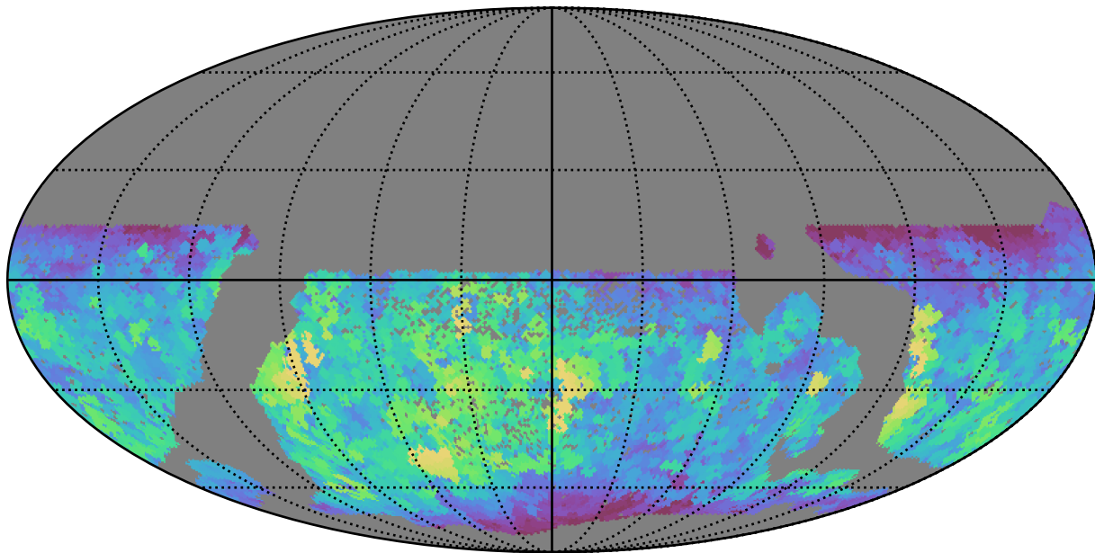
smc_lmc_v3.3_10yrs WFD i band: Max saturation_mag
