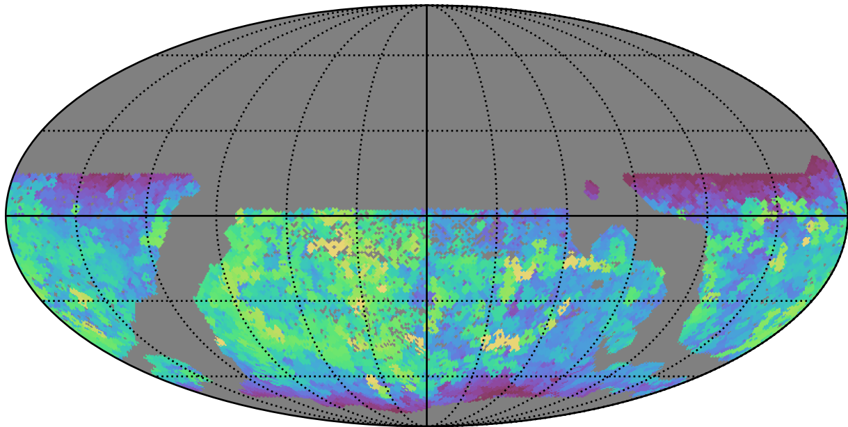
smc_lmc_v3.3_10yrs WFD all bands: Max saturation_mag
