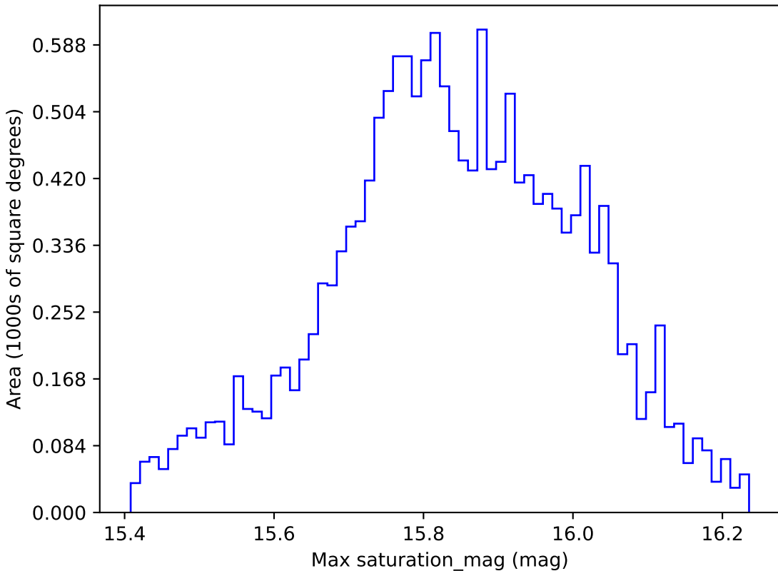
smc_lmc_v3.3_10yrs WFD all bands: Max saturation_mag
