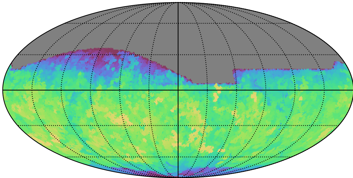
smc_lmc_v3.3_10yrs All sky z band: Max saturation_mag
