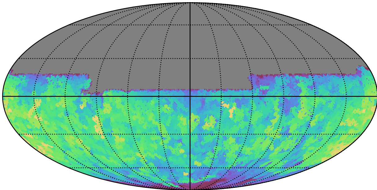
smc_lmc_v3.3_10yrs All sky u band: Max saturation_mag
