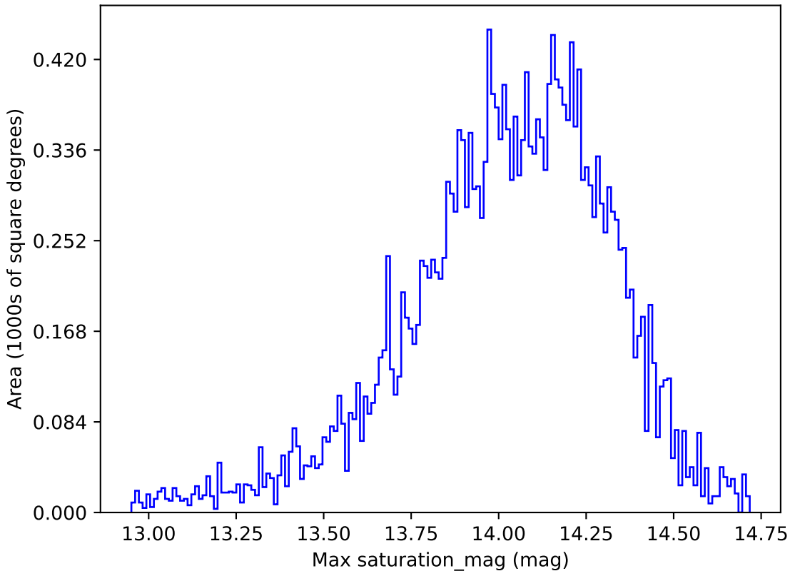
smc_lmc_v3.3_10yrs All sky u band: Max saturation_mag
