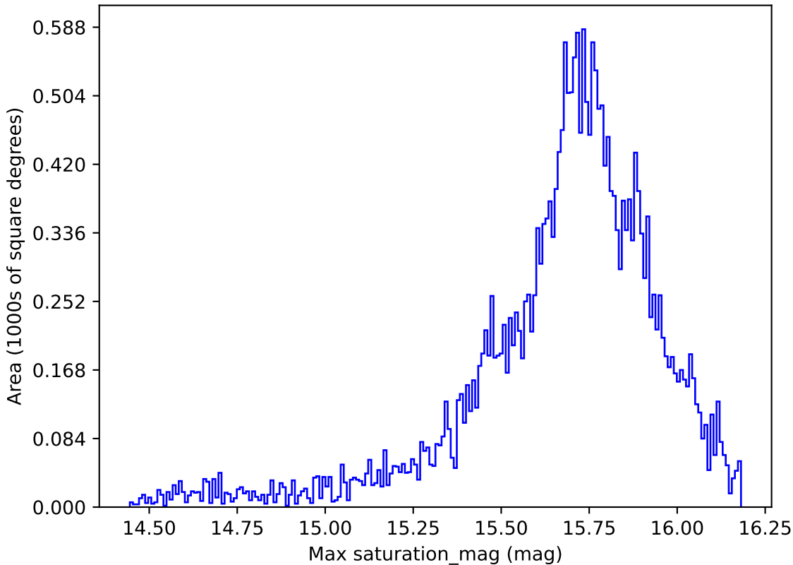
smc_lmc_v3.3_10yrs All sky r band: Max saturation_mag
