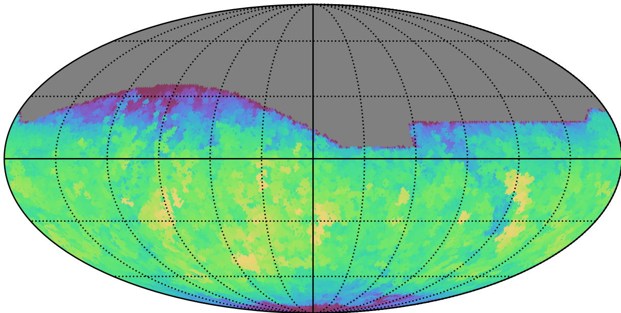
smc_lmc_v3.3_10yrs All sky i band: Max saturation_mag
