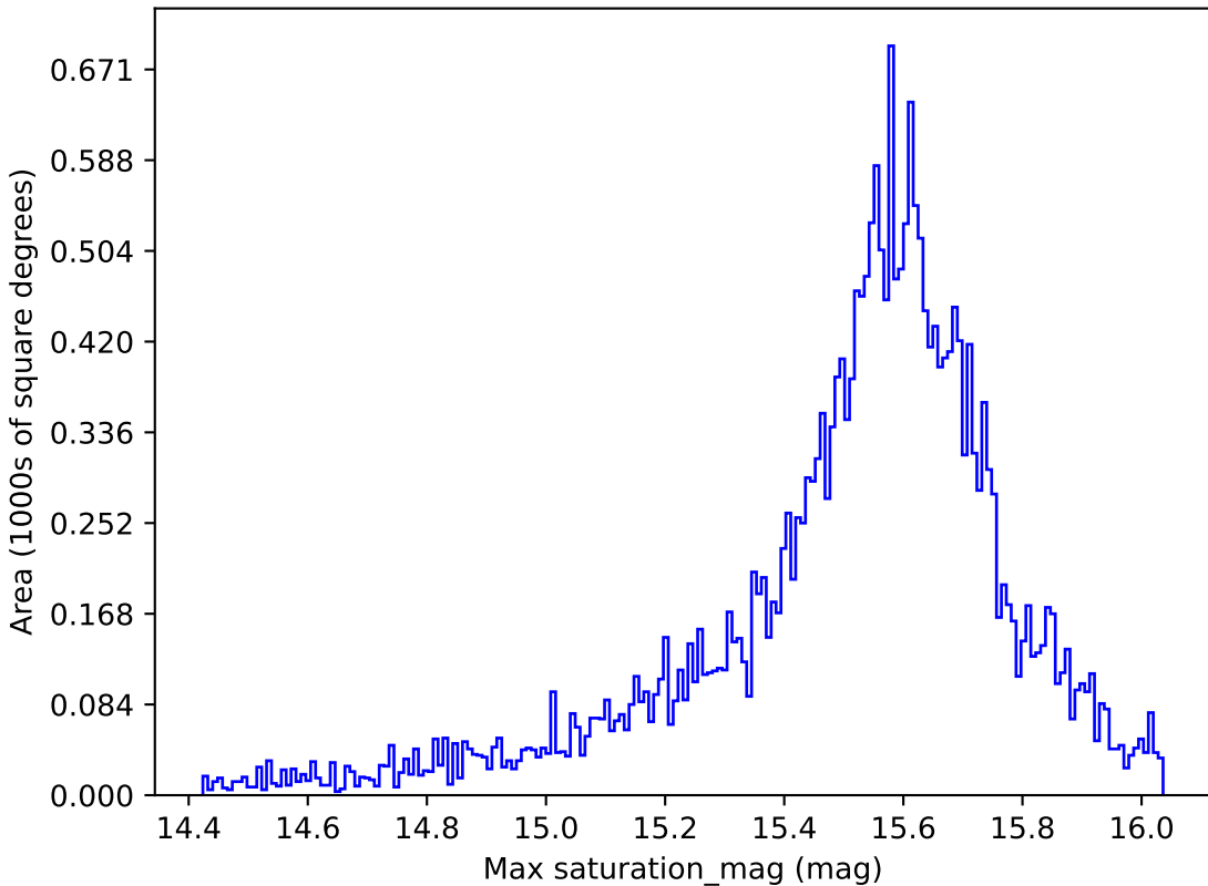
smc_lmc_v3.3_10yrs All sky i band: Max saturation_mag
