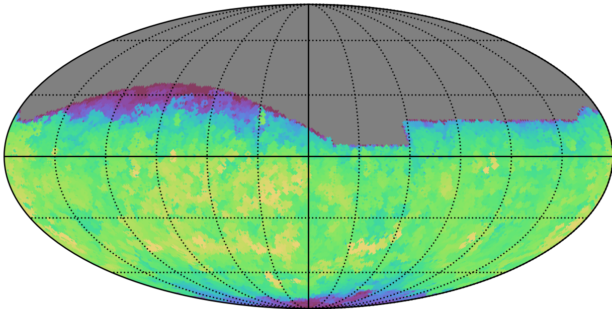
smc_lmc_v3.3_10yrs All sky g band: Max saturation_mag
