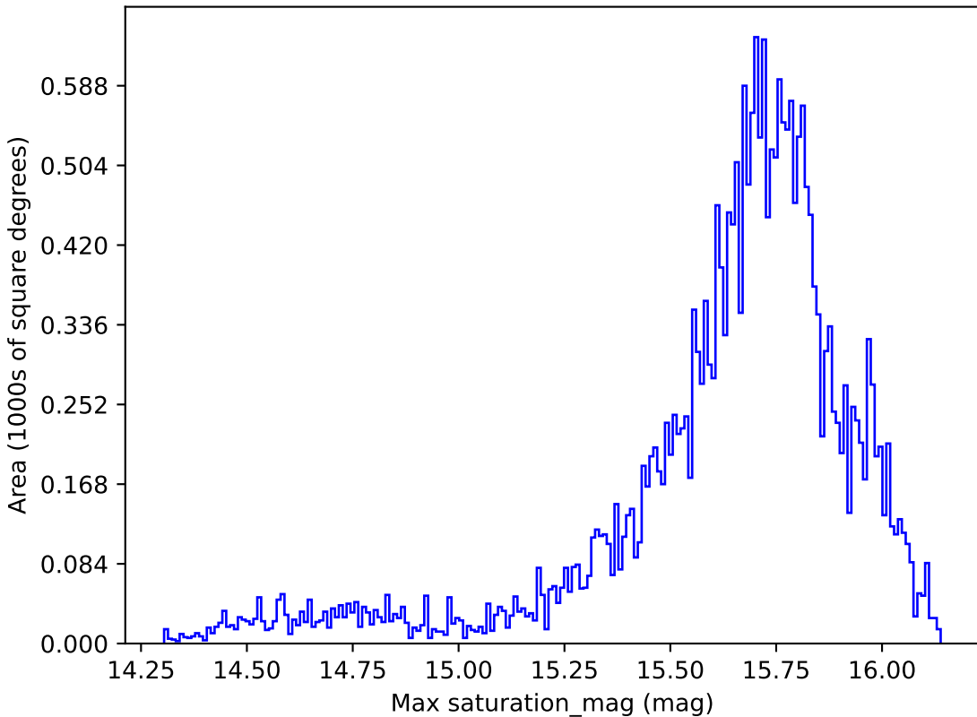
smc_lmc_v3.3_10yrs All sky g band: Max saturation_mag
