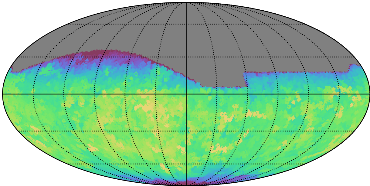
smc_lmc_v3.3_10yrs All sky all bands: Max saturation_mag
