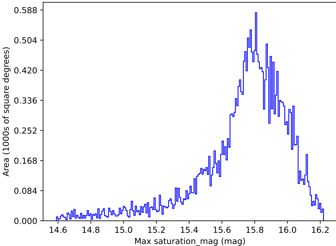
smc_lmc_v3.3_10yrs All sky all bands: Max saturation_mag
