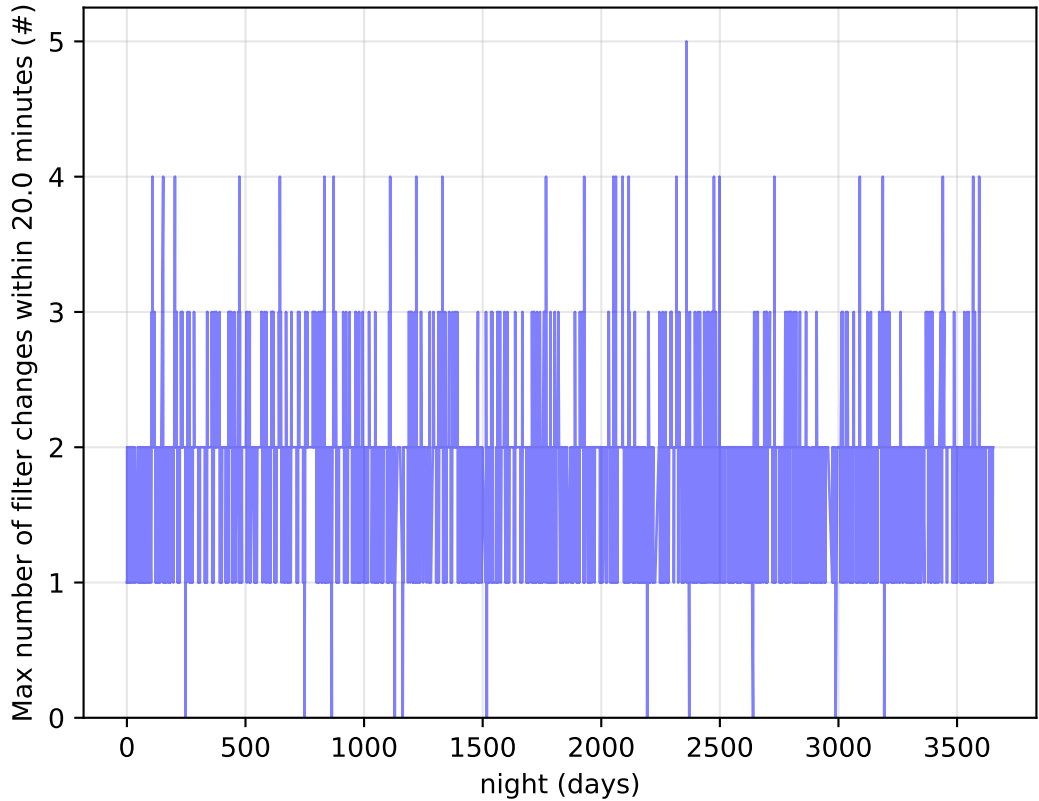
smc_lmc_v3.3_10yrs Per Night: Max number of filter changes within 20.0 minutes
