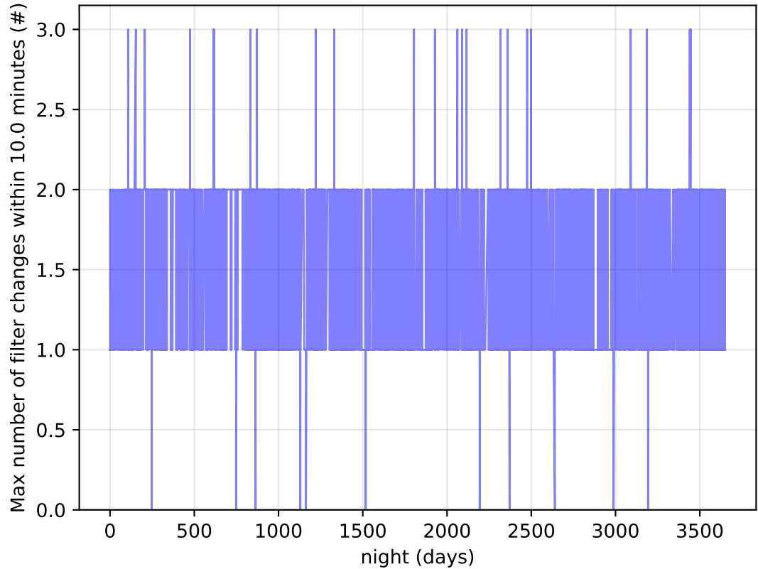
smc_1mc_v3.3_10yrs Per Night: Max number of filter changes within 10.0 minutes
