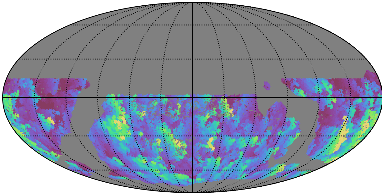
smc_lmc_v3.3_10yrs WFD u band: Max normairmass
