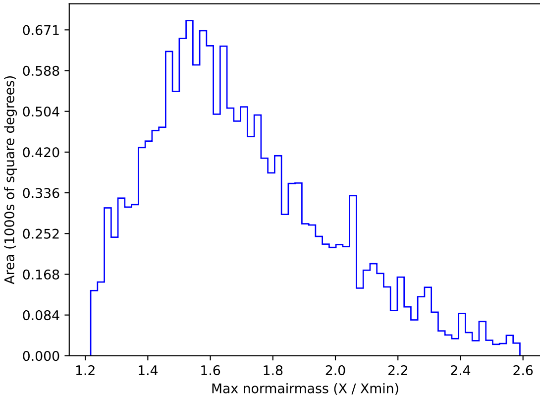
smc_lmc_v3.3_10yrs WFD u band: Max normairmass
