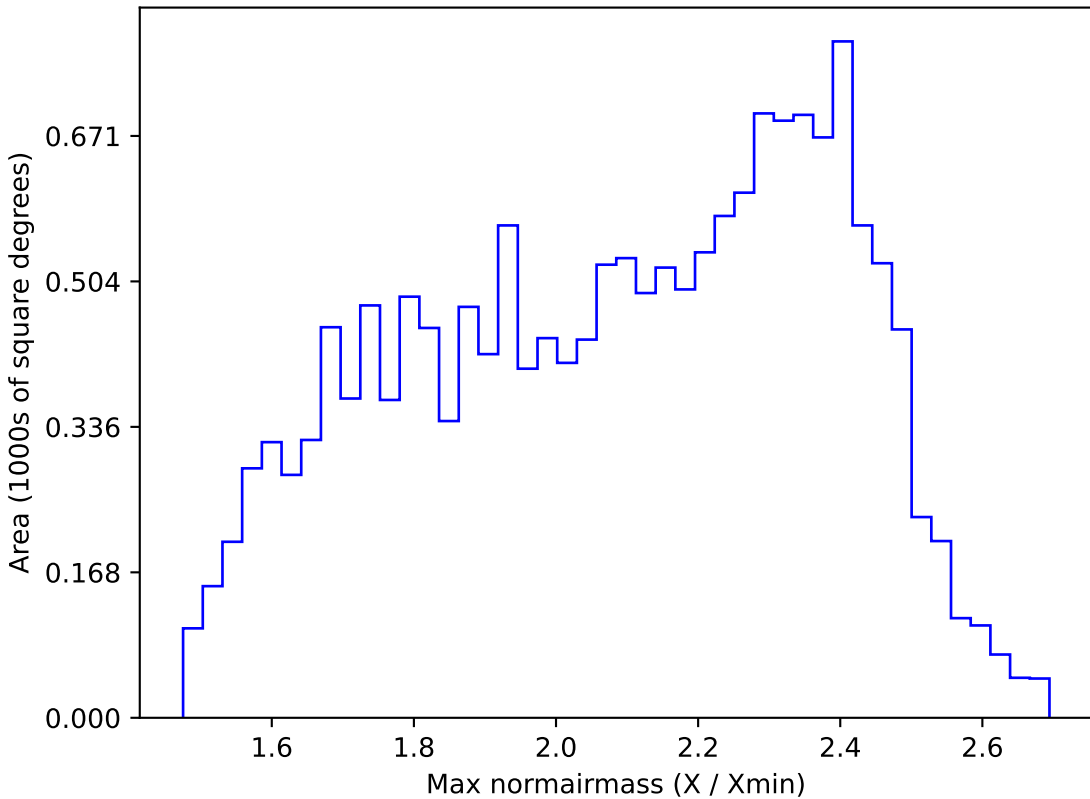
smc_lmc_v3.3_10yrs WFD r band: Max normairmass
