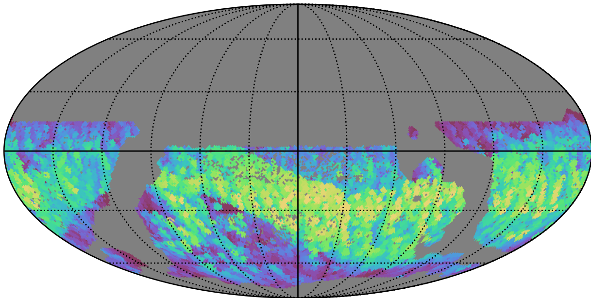
smc_lmc_v3.3_10yrs WFD i band: Max normairmass
