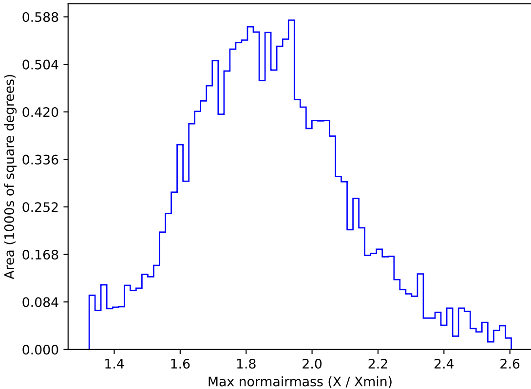
smc_lmc_v3.3_10yrs WFD g band: Max normairmass
