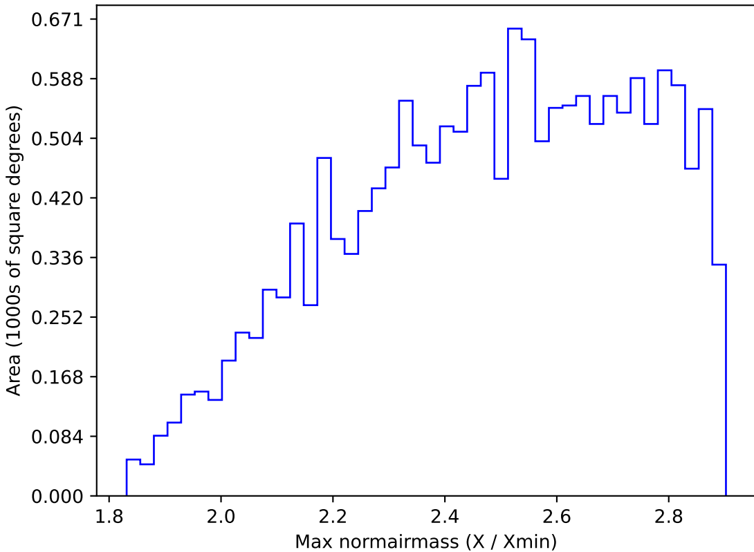
smc_lmc_v3.3_10yrs WFD all bands: Max normairmass
