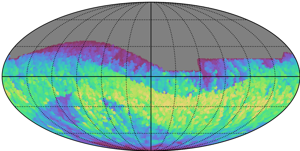
smc_lmc_v3.3_10yrs All sky z band: Max normairmass
