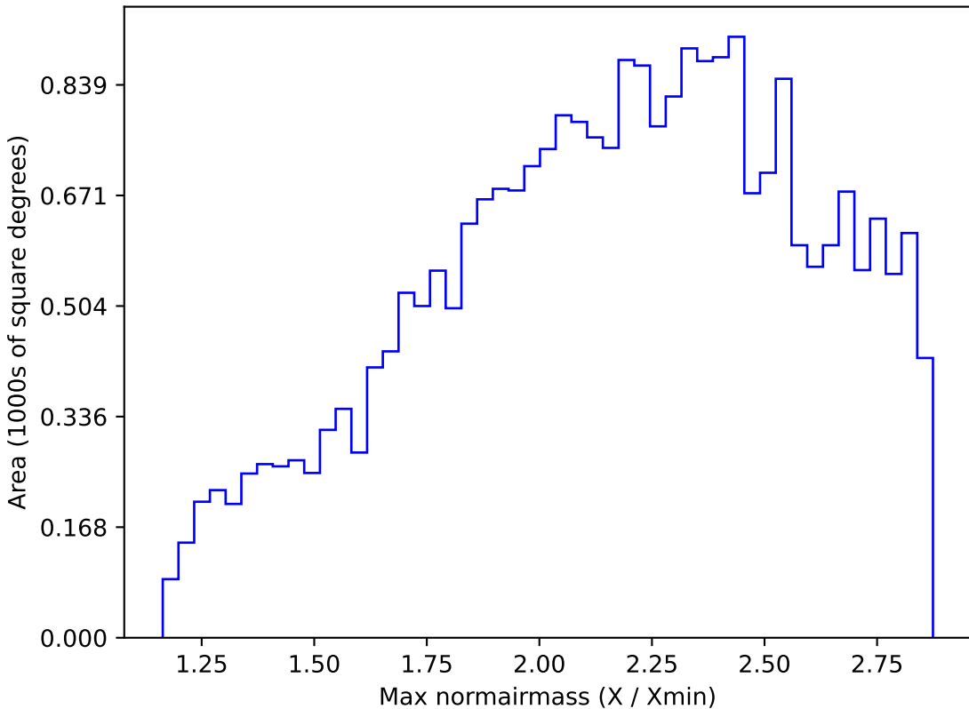
smc_lmc_v3.3_10yrs All sky z band: Max normairmass
