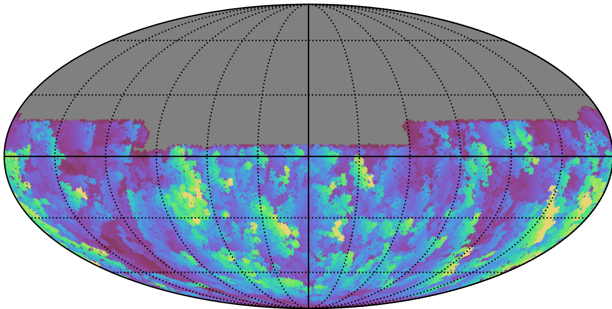
smc_lmc_v3.3_10yrs All sky u band: Max normairmass
